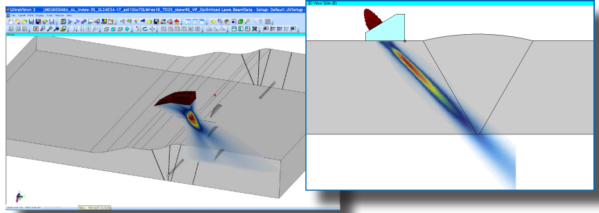
3D beam simulation on complex specimen with Flexible probe
