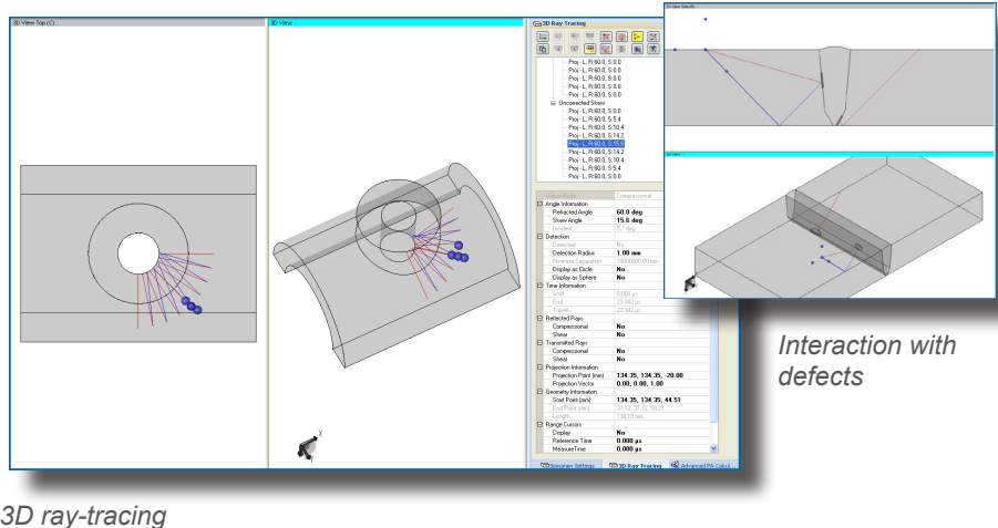
3D ray-tracing
