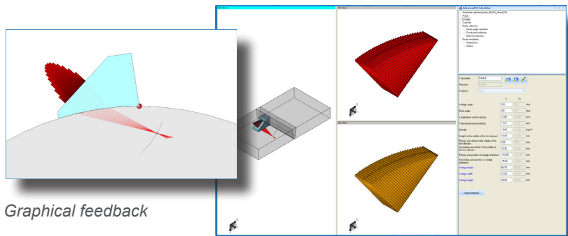
3D beam simulation on complex specimen with Flexible probe
