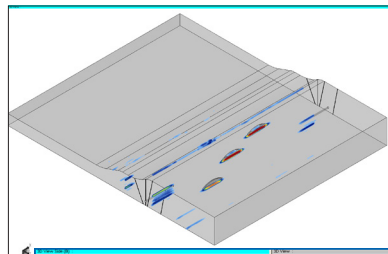
Pipe butt weld data in 3D
