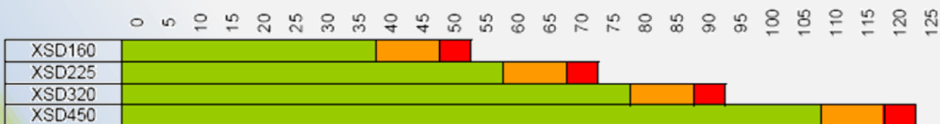
Recommended Steel thicknesses per XSD - SFD700 - OptD 2 - Film ISO 320 - Simple film
